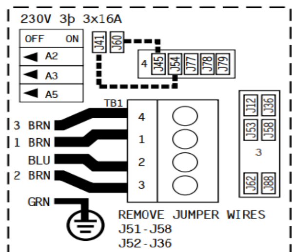
Cablage triphase (3 x 16 amps)
